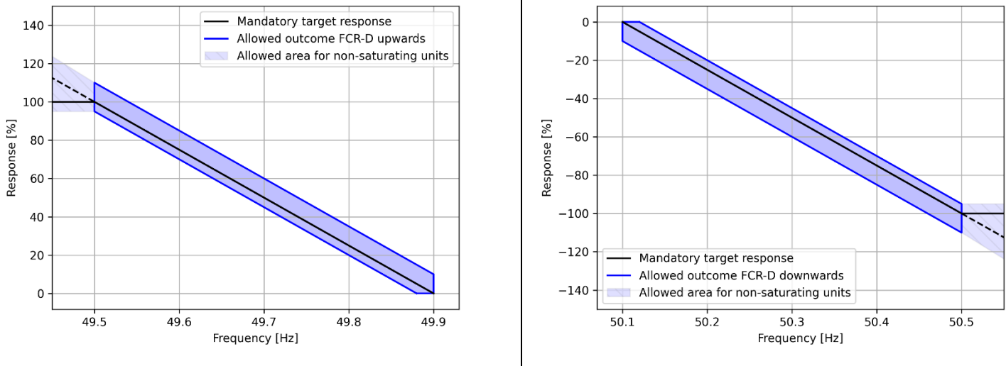
Figure 14 - Activation of piecewise linear FCR-D resources. The black line indicates the mandatory target response, and the blue area defines the allowed outcome of the deviations.
