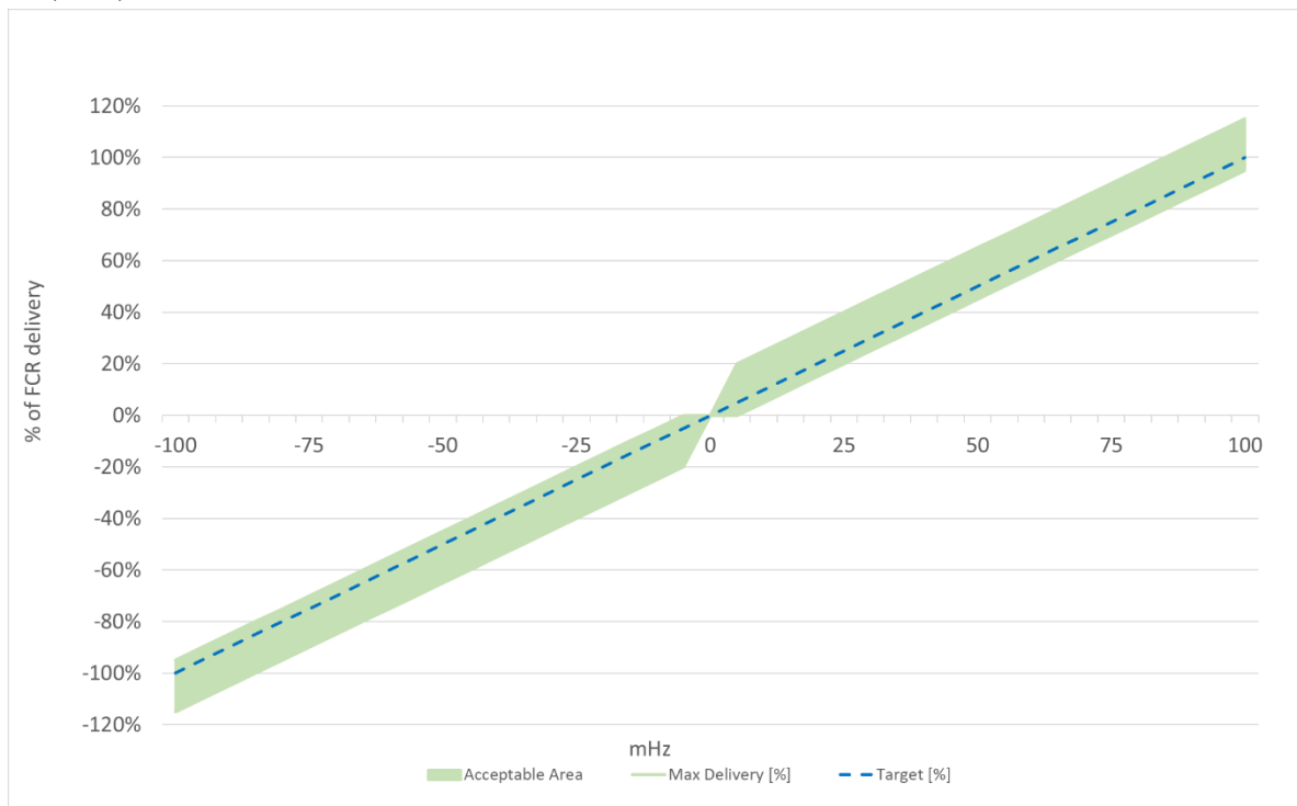
Figure 17 - Activation frequencies for FCR-N ranging with \pm 100 mHz from 50 Hz.
