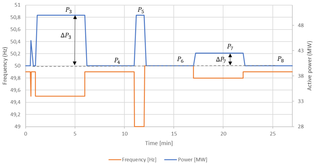
Figure 7 - FCR-D dynamic upwards fast ramp test. FCR-N is omitted in this illustration.
