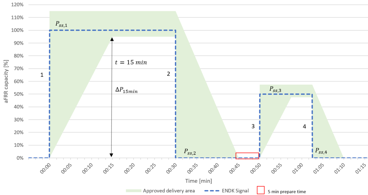
Figure 30 - aFRR functional test response (DK1).
