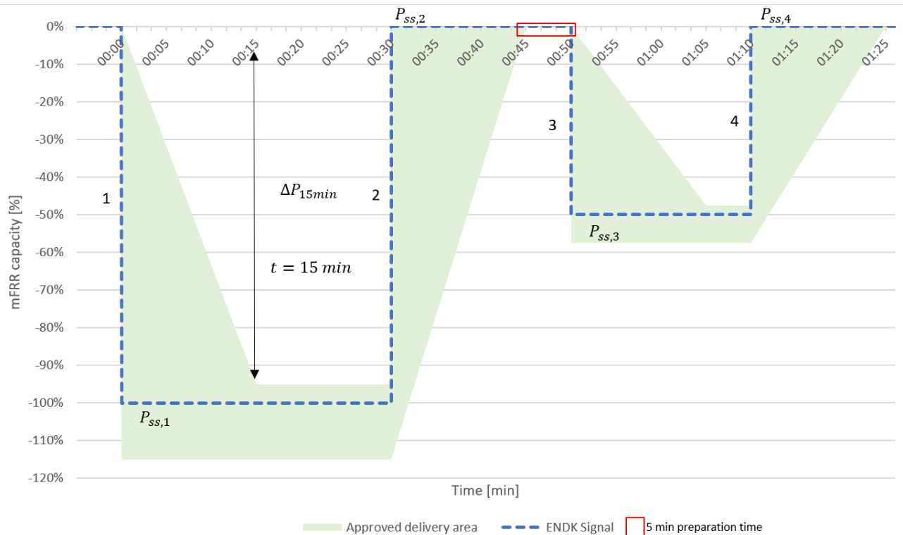
Figure 29 outline the specifics for the up and down direction, respectively. Table 48 describes the exact ramps to effectuate. Table 48 dictates the requirements to obey for the unit when performing the mFRR response test.
