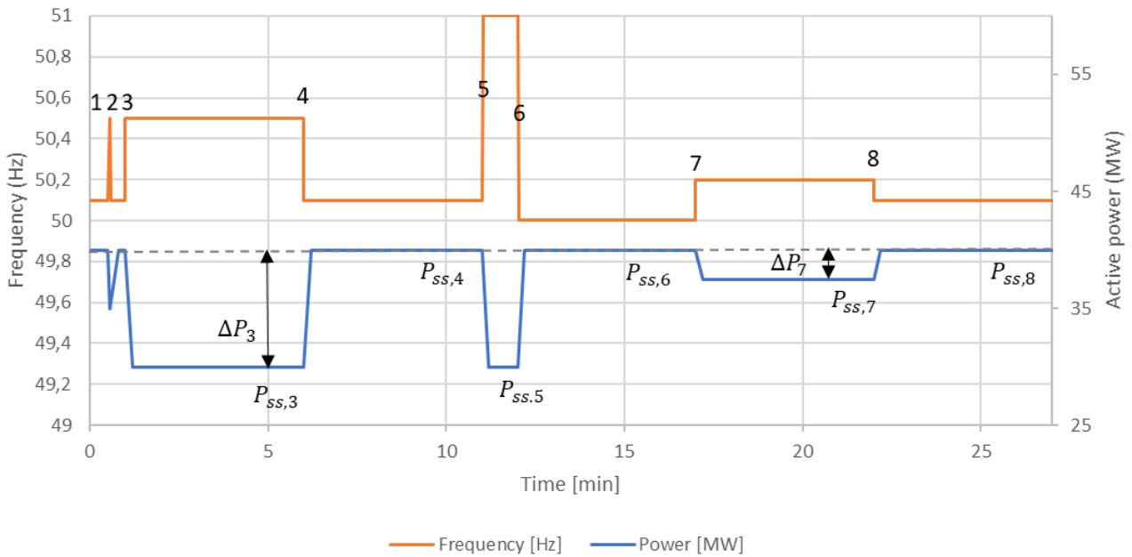
Figure 6 - FCR-D dynamic downwards fast ramp test. FCR-N is omitted in this illustration.
