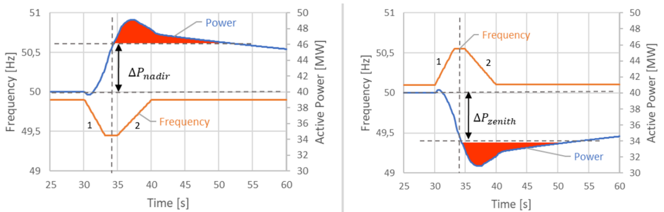
Figure 9 - Deactivation test on ramp 1 and 2 for FCR-D dynamic upwards (left) and FCR-D dynamic downwards (right).
