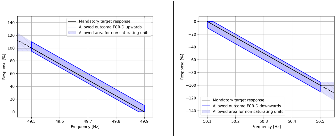
Figure 13 - Activation of piecewise linear FCR-D resources. The black line indicates the mandatory target response, and the blue area defines the allowed outcome of the deviations.
