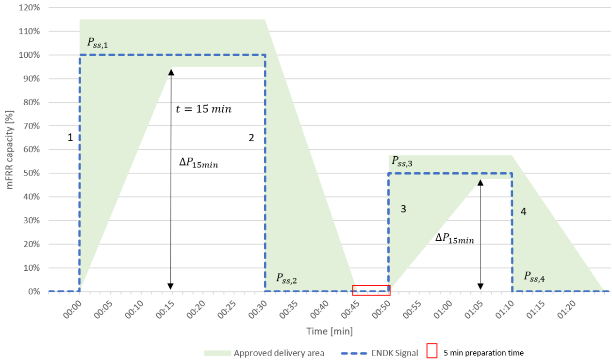
Figure 28 - Tests of minimum requirements for response for mFRR at upwards regulation.
