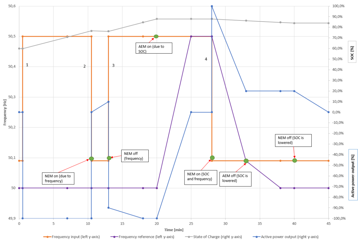
Figure 16 Energy management test of FCR-D downwards, steps 1-4. NOTE: This is an example. Hence, NEM/AEM activations will vary dependent on specific MW/MWh capacities of the LER unit.
