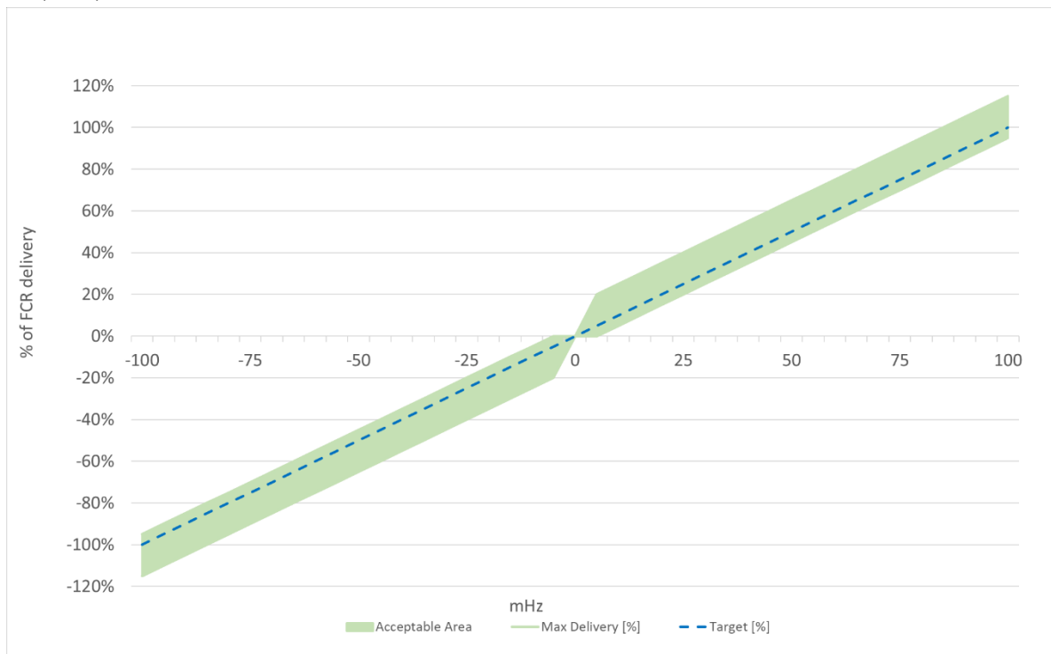
Figure 17 - Activation frequencies for FCR-N ranging with +/- 100 mHz from 50 Hz.
