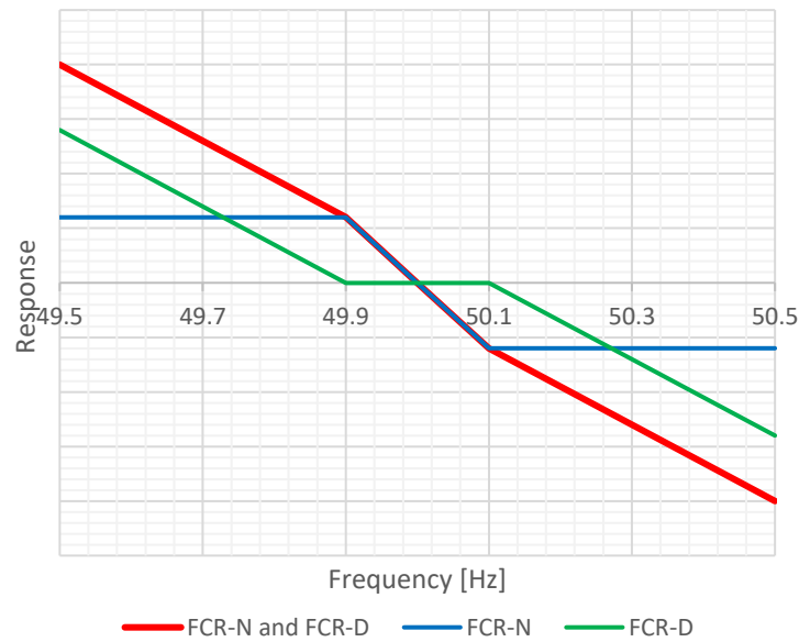
Figure 10 - Steady state active power activation as a function of frequency, droop profile of FCR-N (blue), FCR-D (green) and both combined (red).
