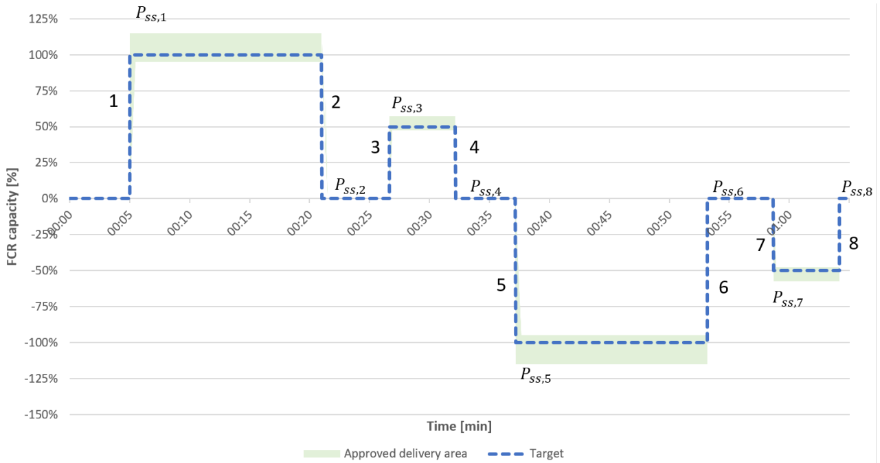
Figure 2 - Tests of minimum requirements for response for FCR at both upward and downward regulation (DK1).
