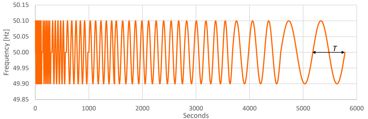
Figure 19 - illustrates the full FCR-N sine test without breaks.
