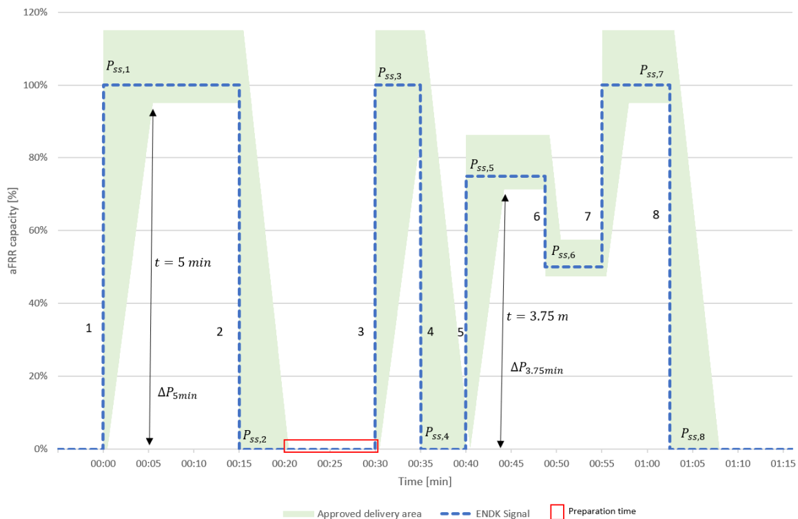
Figure 31 - aFRR functional test response (DK2).
