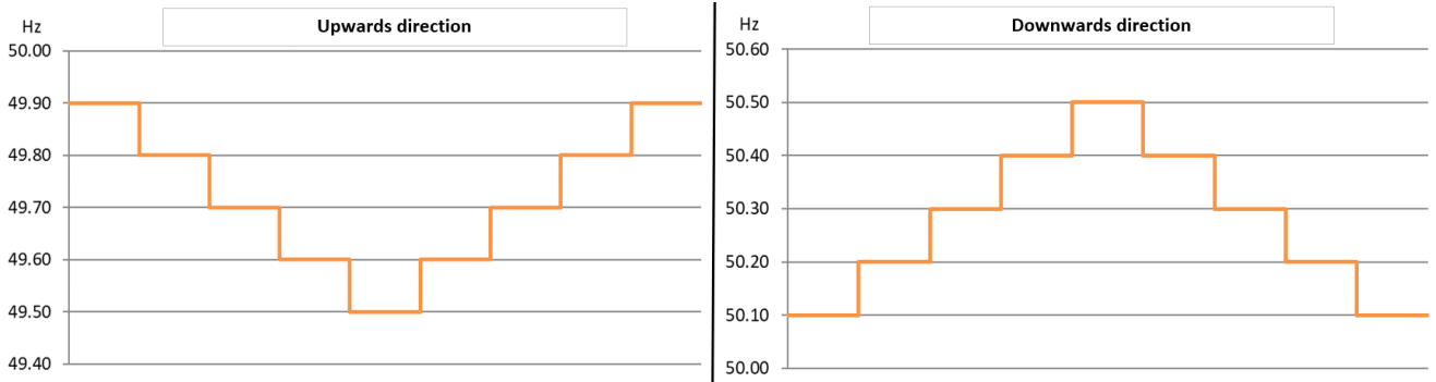
Figure 14 - FCR-D up- (left part) and downwards (right part) linearity test sequence.
