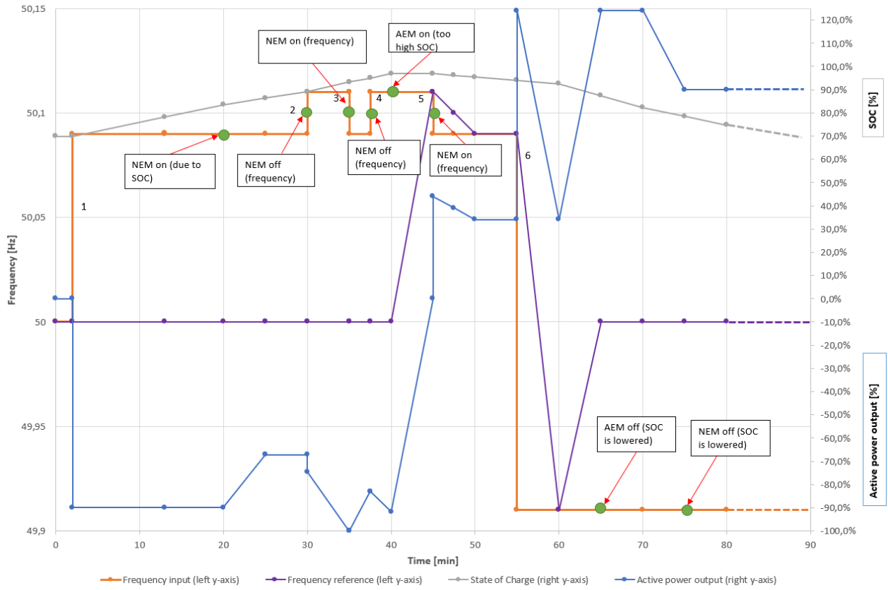
Figure 23 Energy management test of FCR-N, steps 1-6. NOTE: This is an example. Hence, NEM/AEM activations will vary dependent on specific MW/MWh capacities of the LER unit
