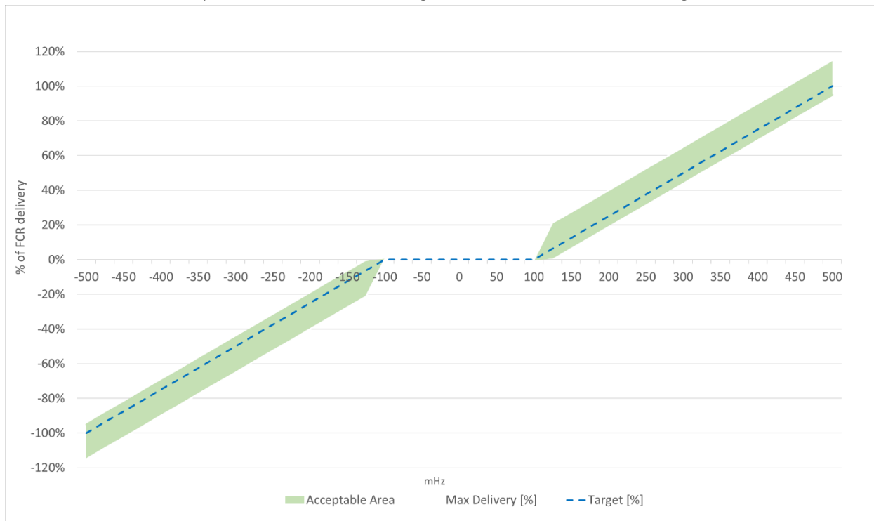
Figure 5 - Activation frequencies for FCR-D ranging with \pm 400 mHz from 49.9 and 50.1 Hz.
