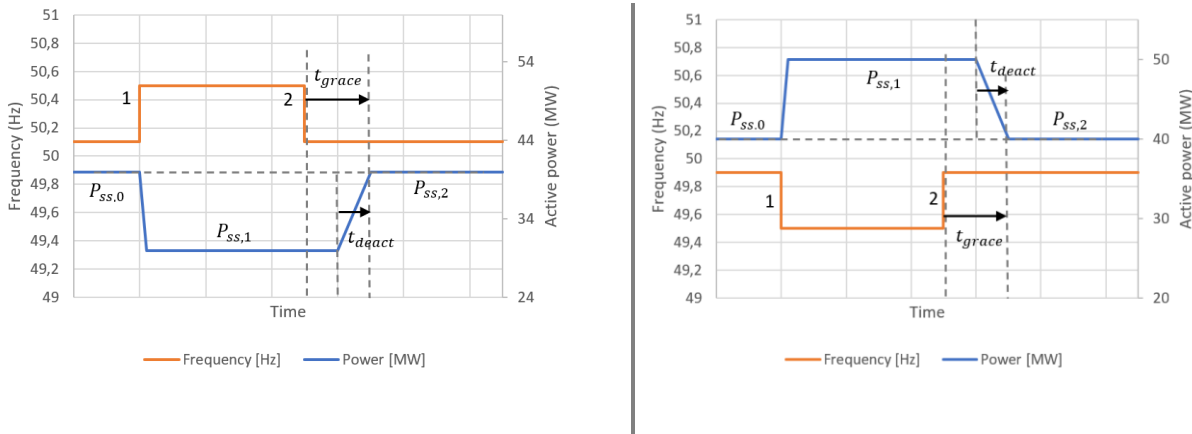
Figure 12 - FCR-D static downwards (left) and upwards (right) ramp test. FCR-N is omitted in this illustration.
