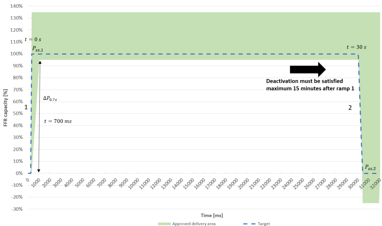
Figure 24 FFR response sequence for Alternative 2 in Table 46 (0.7s reaction time, 30s steady state response, instantaneous deactivation at ramp 2).
