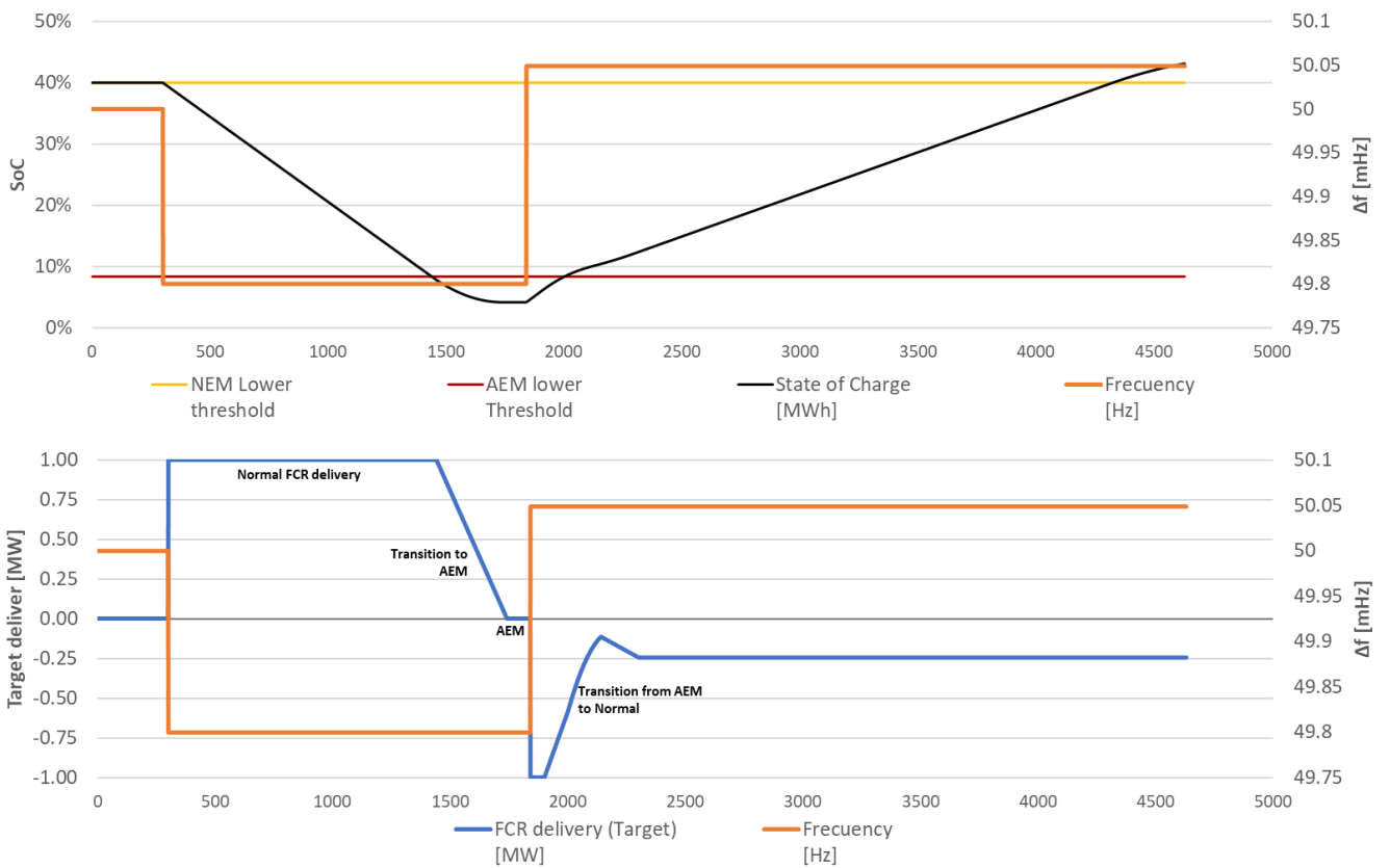
Figure 4 – Visual demonstration of energy management for FCR.
