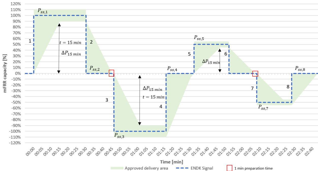
Figure 27 - Tests of minimum requirements for response for mFRR at both upward and downward regulation.
