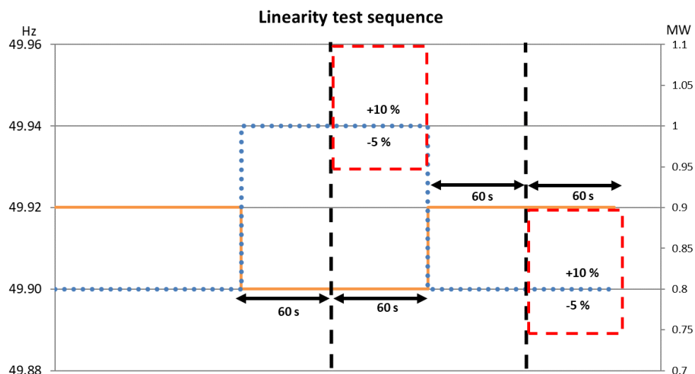
Figure 22 - Allowed response area for FCR-N for the frequency steps from 49.92 Hz \rightarrow 49.90 Hz \rightarrow 49.92 Hz. The orange line is the frequency step. The blue dotted line is the directly proportional FCR response. The red dashed squares indicate the allowed response area, denoted to assess the FCR response for 60 seconds.
