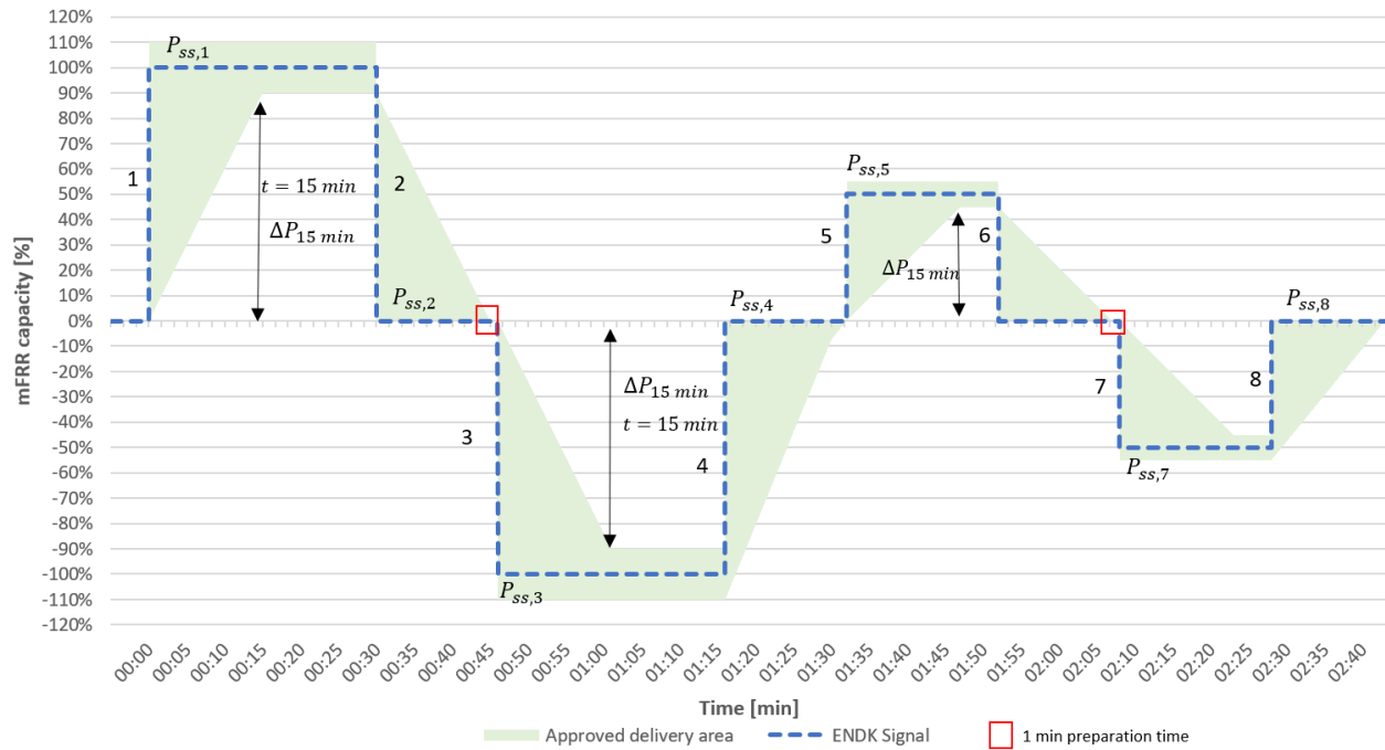
Figure 27 specifies the mFRR test sequence to perform when a prequalification for both up and downregulation is desired. Thus, upward and downward regulation should be delivered at full and part load. Table 47 describes the exact ramps to effectuate.
