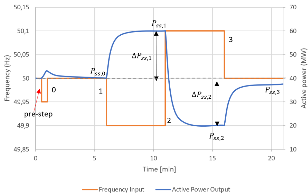
Figure 18 - FCR-N step response sequence.
