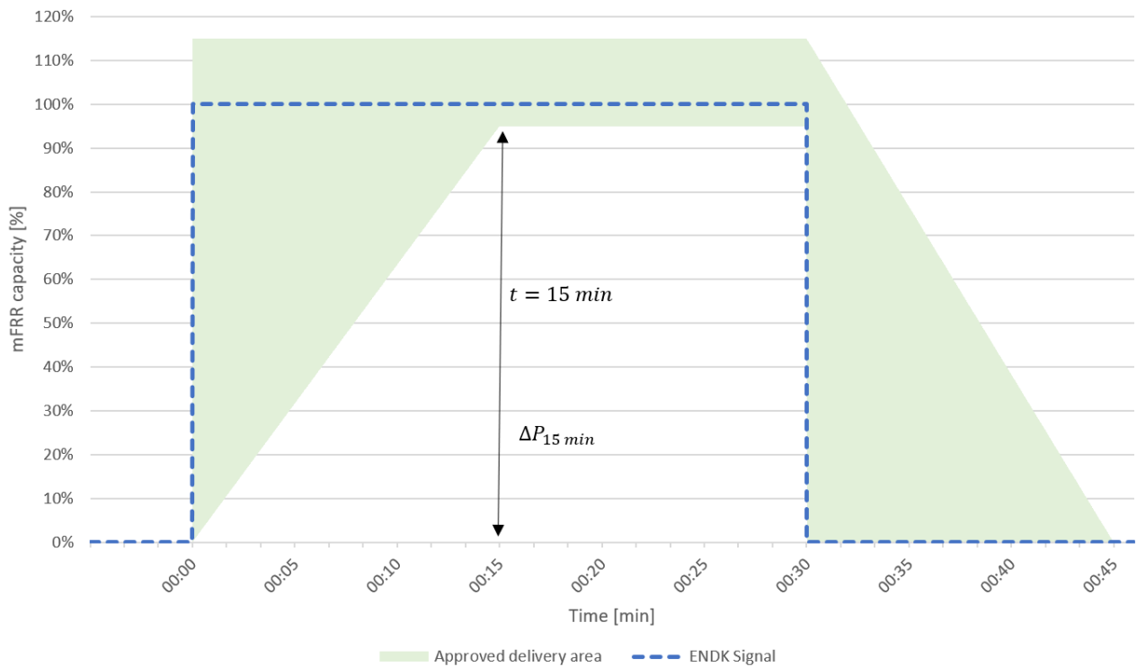
Figure 26 - mFRR activation response sequence, denoting a full response at 15 minutes.
