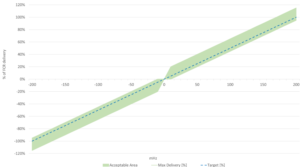
Figure 1 - Power response from FCR including the accepted tolerance area.
