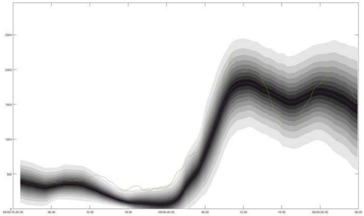
Figure 32 – Graphic illustration of application of 10% percentile in a probabilistic prognosis to estimate available capacity at the time of bidding for mFRR (9 o'clock, D-1).
