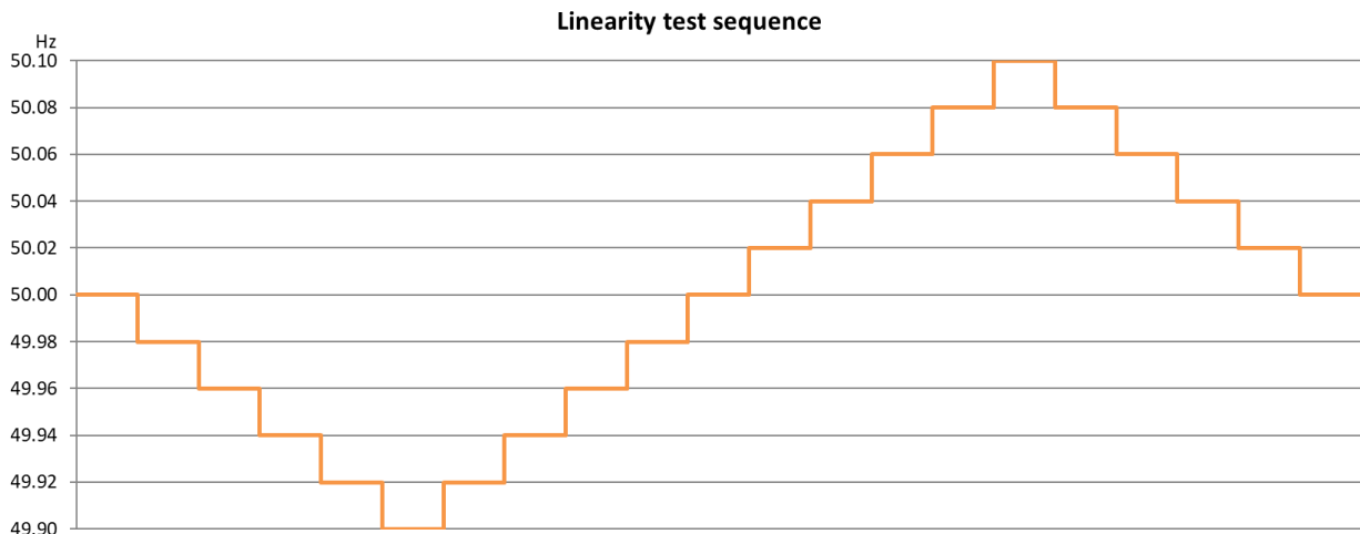
Figure 21 - FCR-N linearity test sequence.
