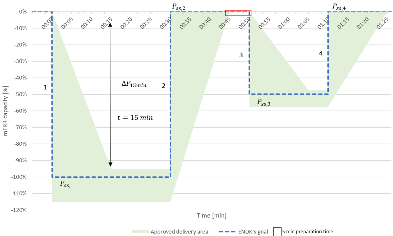
Figure 29 - Tests of minimum requirements for response for mFRR at downwards regulation.
